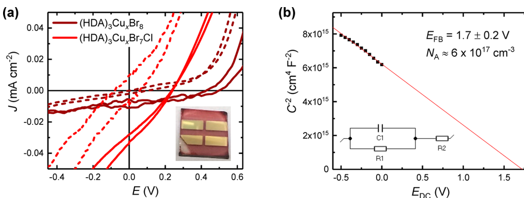
Figure 7. (a) J-E behavior for solar cells consisting of Au/spiro-OMeTAD/Cu/ \text{TiO}_2 /FTO, where Cu stands for (\text{HDA})_3\text{Cu}_x\text{Br}_8 or (\text{HDA})_3\text{Cu}_x\text{Br}_7\text{Cl} . Solid lines represent measurements under 1 sun irradiance, and dashed lines represent dark measurements. Inset: digital photograph image of a complete solar cell. (b) Impedance spectroscopy data, presented as a Mott–Schottky plot, for a solar cell consisting of Au/spiro-OMeTAD/ (\text{HDA})_3\text{Cu}_x\text{Br}_7\text{Cl} / \text{TiO}_2 /FTO and with the calculated flat-band potential ( E_{FB} ) and dopant density ( N_A ). Inset: standard Randles circuit used to model the impedance spectroscopy data.
