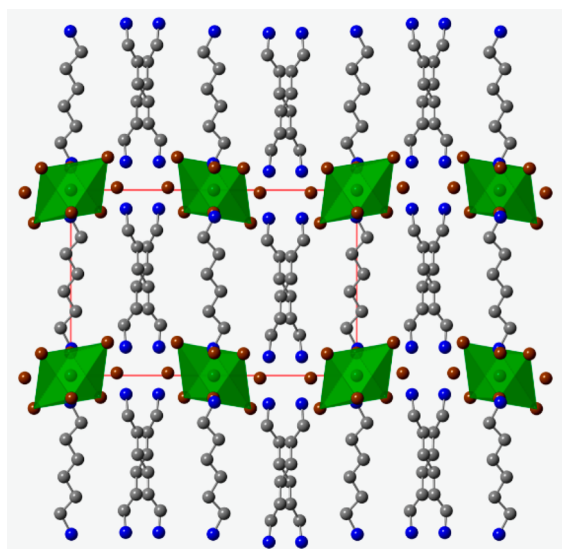
Figure 1. Single-crystal X-ray structure of (\text{HDA})_3\text{CuBr}_8 as seen from the b -axis showing Cu–Br octahedral (green), Cu (green), Br (brown), N (blue), and C (gray). Hydrogen atoms are omitted for clarity.
